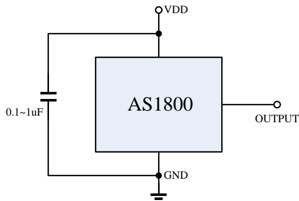
Figure 1, Typical Application Circuit of AS1800
