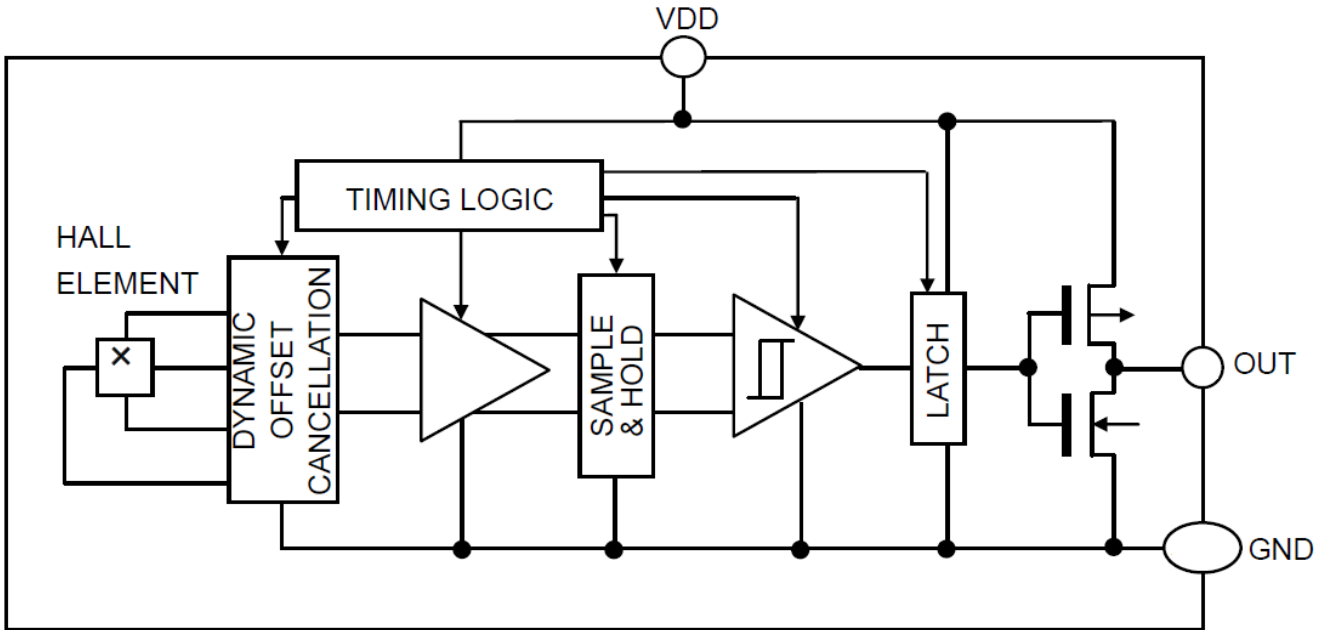
Figure 3, Block Diagram of AS1800
